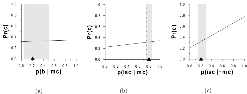
Figure 6.3: A one-way sensitivity analysis of the example Bayesian network.
