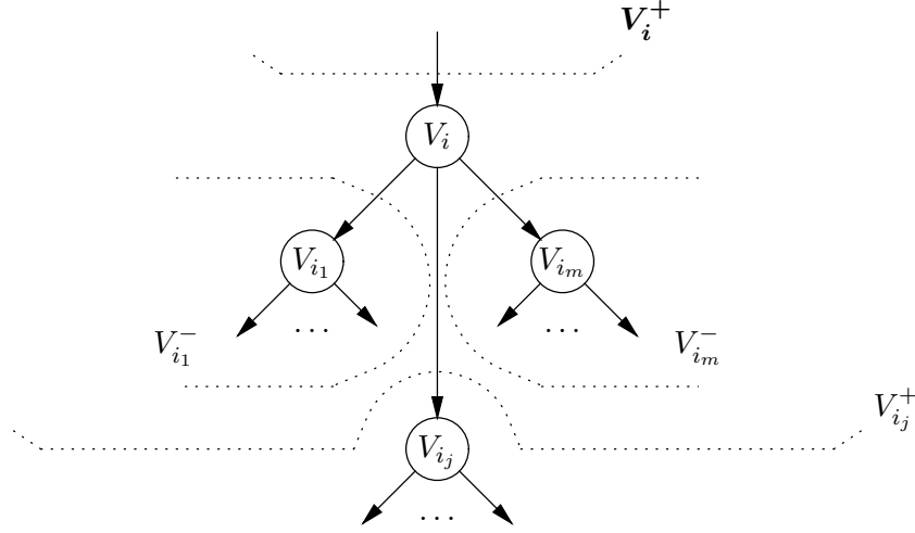
Figure 4.4: Exploiting d-Separation for Computing \pi_{V_{i_j}}^{V_i}(V_i) .
