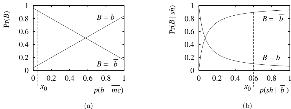
Figure 6.5: The sensitivity functions for the two possible values of the variable of interest B as a function of (a) parameter \gamma(b | \neg mc) , and (b) parameter \gamma(sh | \neg b) , given a severe headache.
