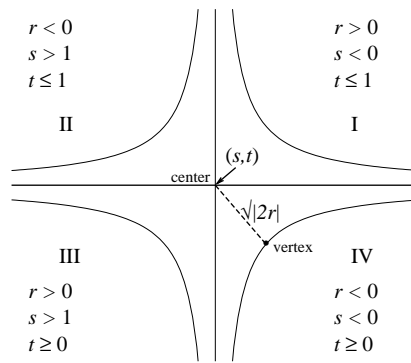
Figure 6.2: Hyperbolas and their constants (the constraints on s and t are specific for sensitivity functions)
