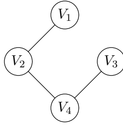
Figure 3.1: An Example Undirected D-map.
