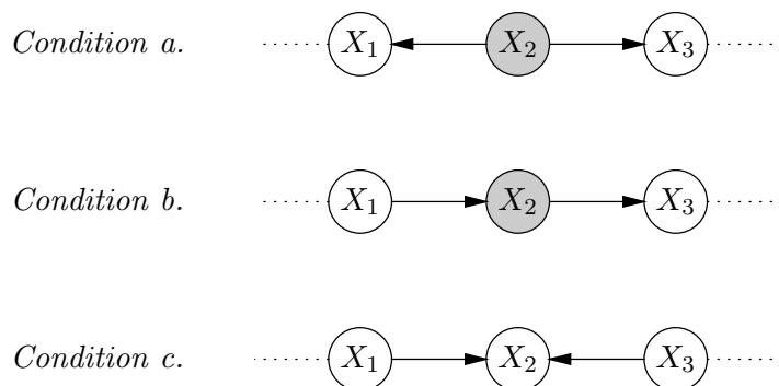
Figure 3.4: Chain Blocking; Shaded Vertices are Members of Blocking-set \mathbf{W} .
