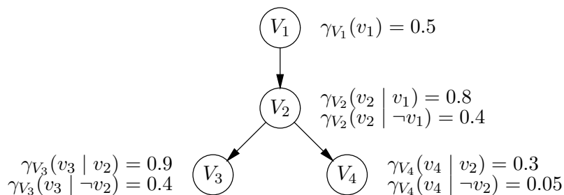
Figure 4.5: An Example Bayesian Network.
