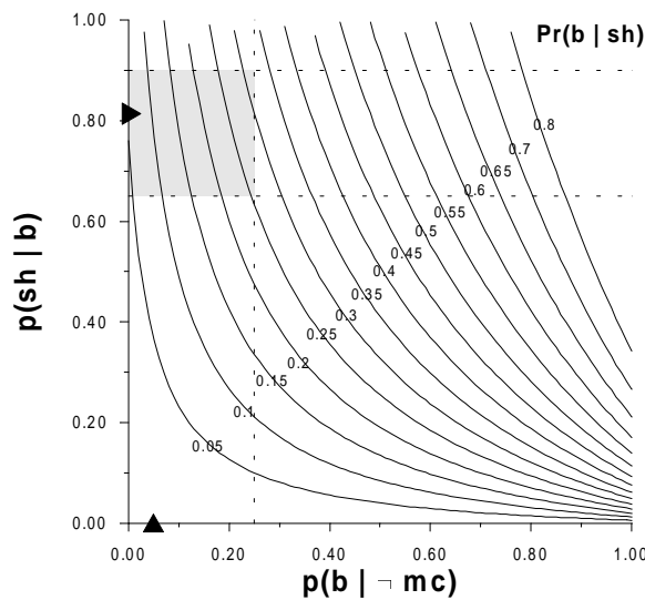
Figure 6.8: A two-way sensitivity analysis of the example Bayesian network.
